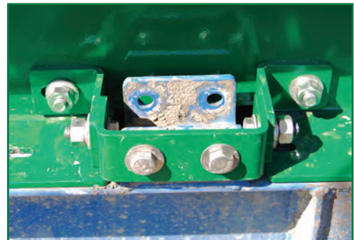
Attach basket to support frame.
